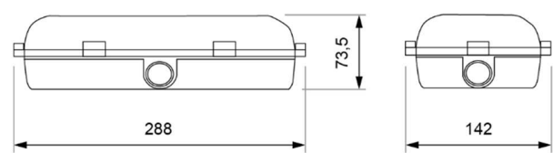
Watertight mounting
